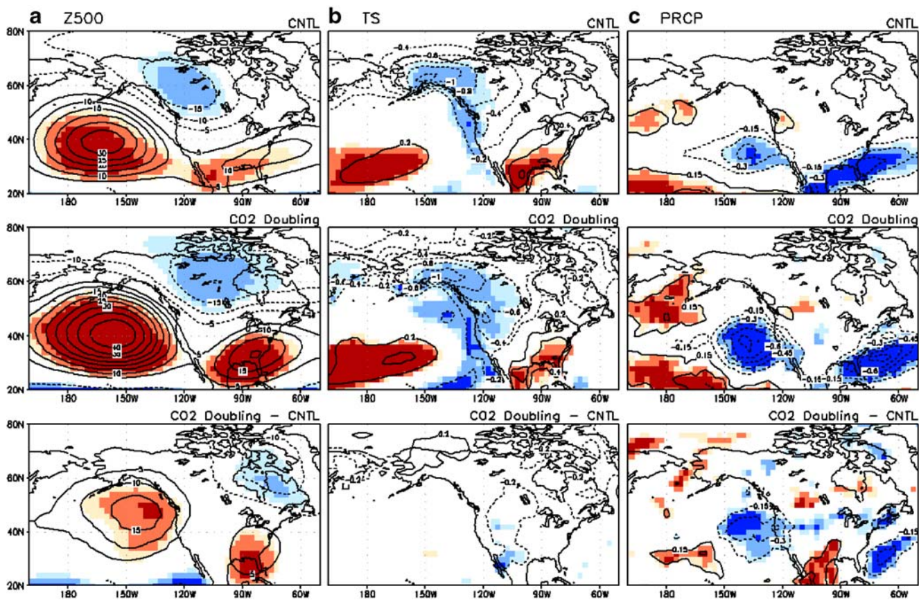
Fig. 5 As in Fig. 4 except for La Niña composite
