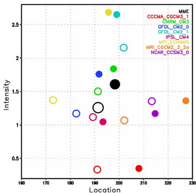
Fig. 3 Scatter plots for the intensity of the maximum precipitation vs. its longitudinal location. Intensity and location are determined based on the linear regression map of the precipitation against the Niño-3.4 index. Open and closed dots are obtained from the control and \text{CO}_2 doubling experiments, respectively
