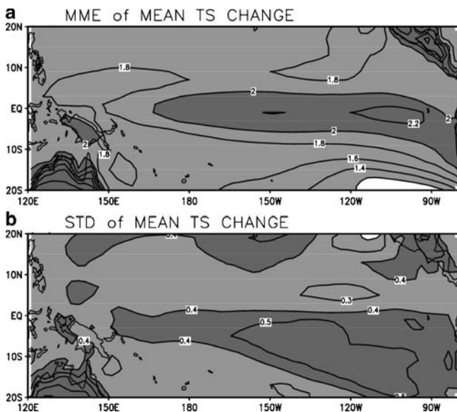
Fig. 1 a Difference in the eight-member multimodel ensemble SST between the control and CO 2 doubling experiments. b Standard deviation of SST difference
