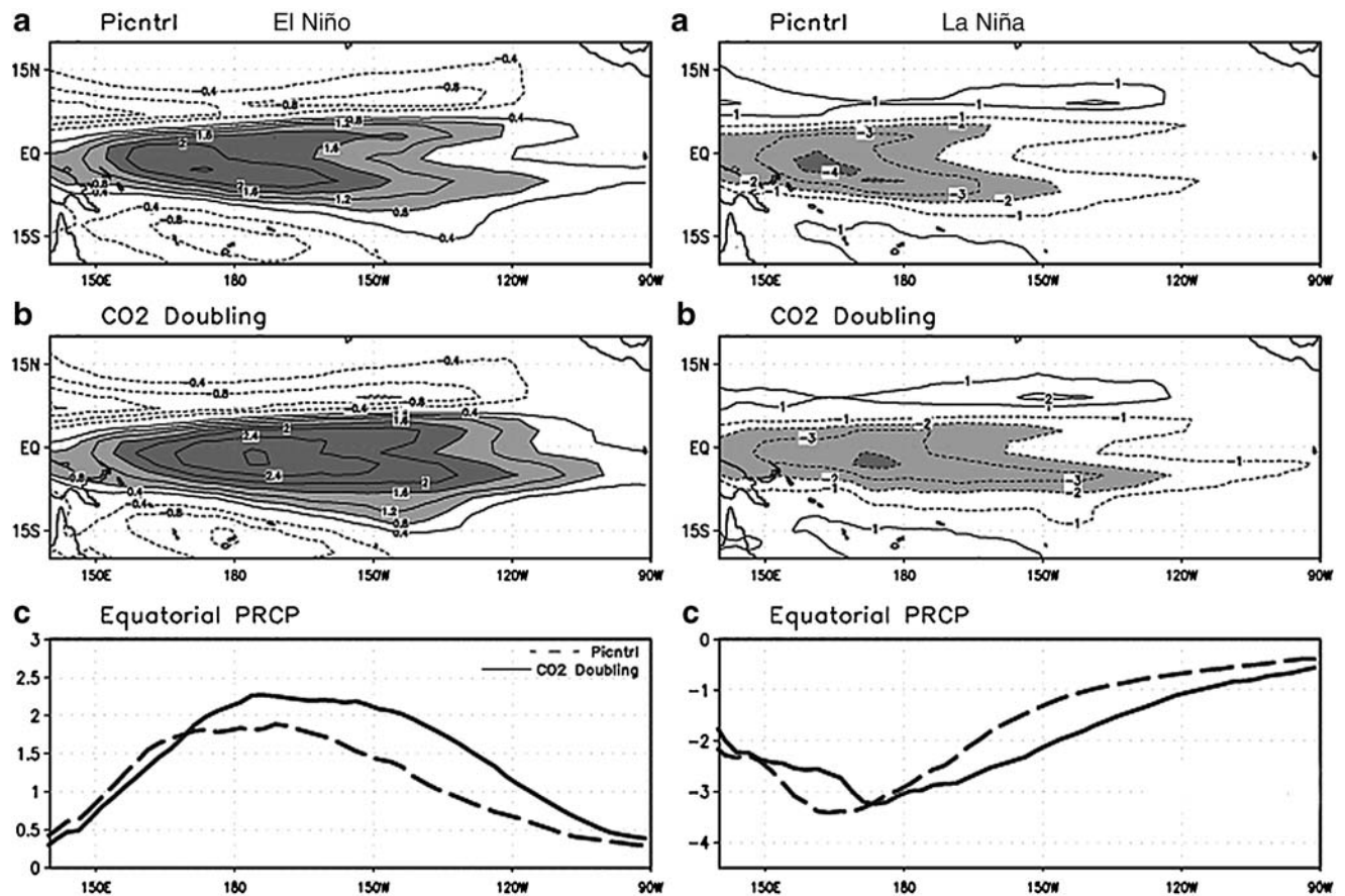
Fig. 2 a Composite map of the precipitation against Niño-3.4 index for the control experiment. b As in a but for the CO 2 doubling experiment. c Equatorial (5° S–5° N) precipitation anomalies for the
