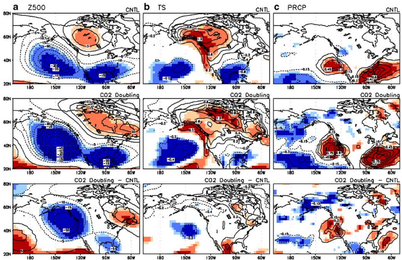
Fig. 4 a El Niño composite map of 500 hPa geopotential height for the control ( upper panel ) and CO 2 doubling ( middle panel ) experiment. b, c As in a but for the surface temperature and precipitation, respectively. Lower panels show the difference between control and
